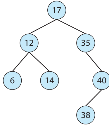
Figure 1.20 Binary search tree.
