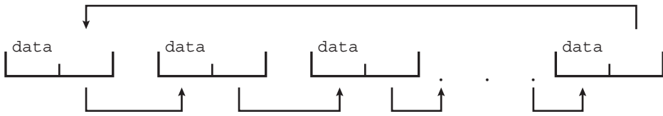
Figure 1.19 Circularly linked list.
