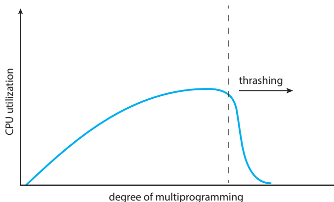
Figure 10.20 Thrashing.
