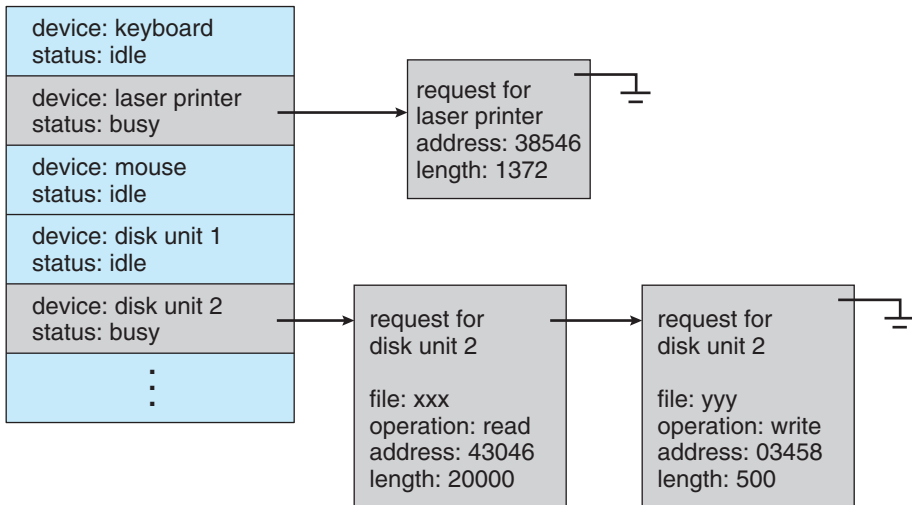
Figure 12.10 Device-status table.
