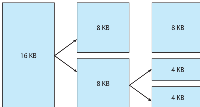
Figure 20.4 Splitting of memory in the buddy system.
