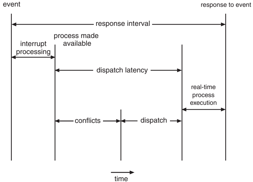
Figure 5.19 Dispatch latency.
