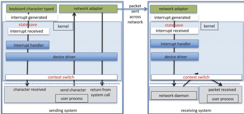
Figure 12.16 Intercomputer communications.
